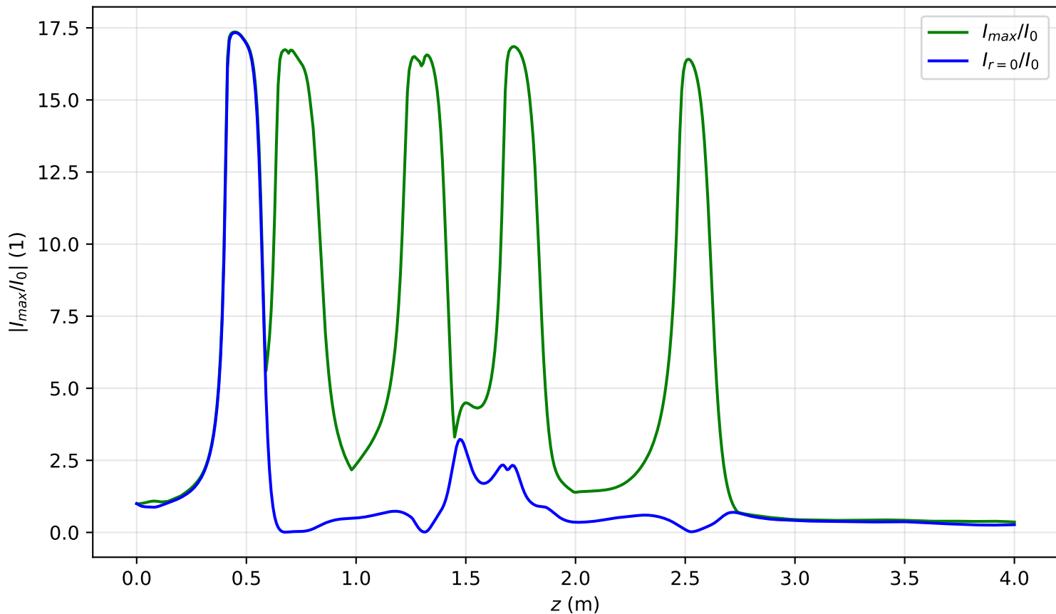
I_{max}(x = 0, y = 0, z)/I_0 , Pin=6.4P_{cr} , noisy input, artificial time
